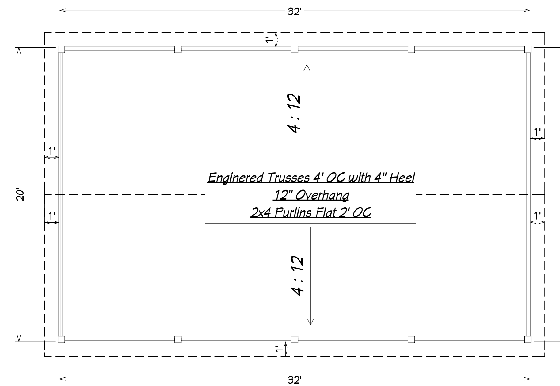
Roof Plan 1/4" Scale
