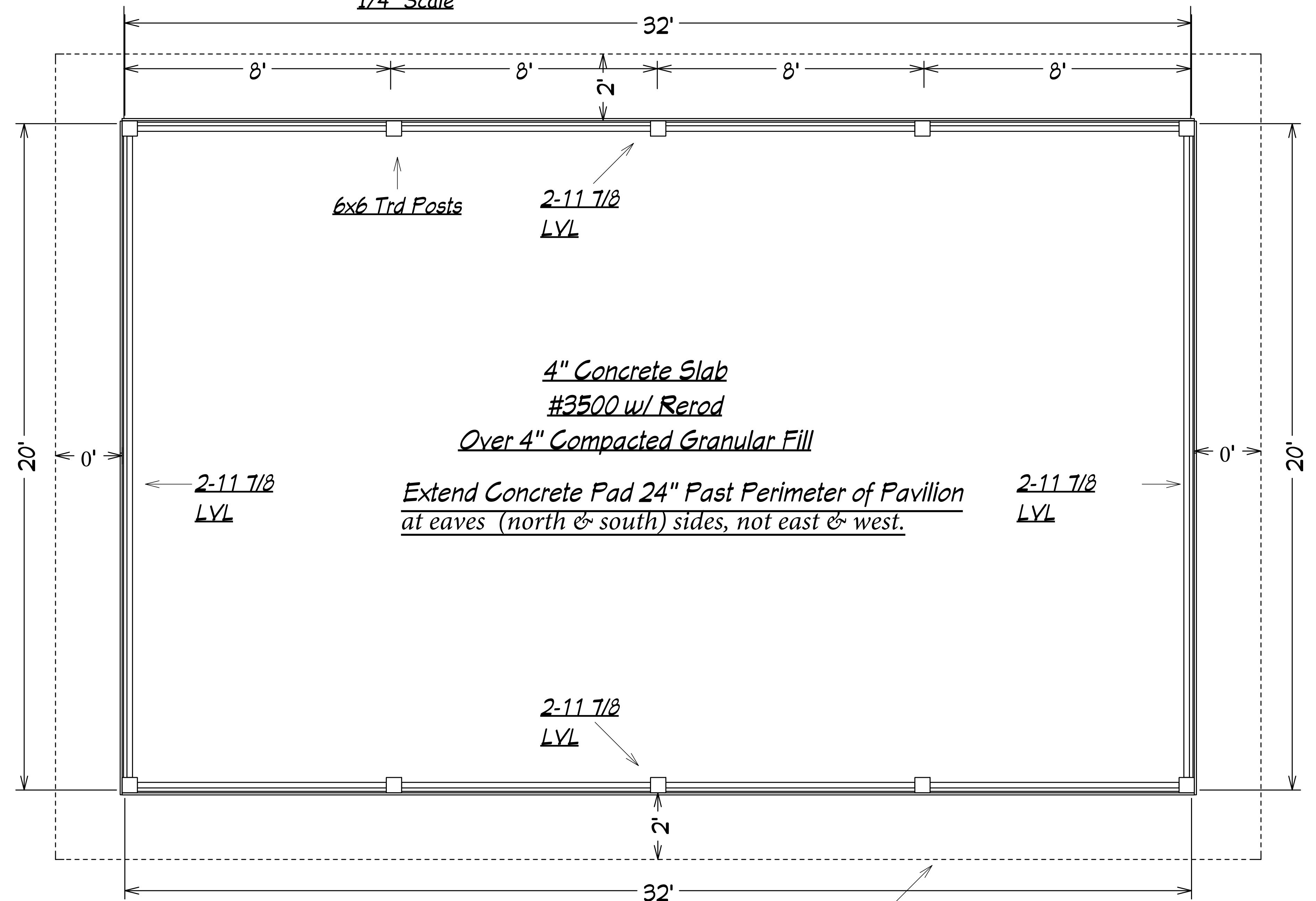
Pavilion Plan 1/2" Scale
